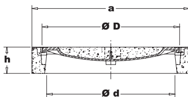
type 7410.10 (B2741010)
